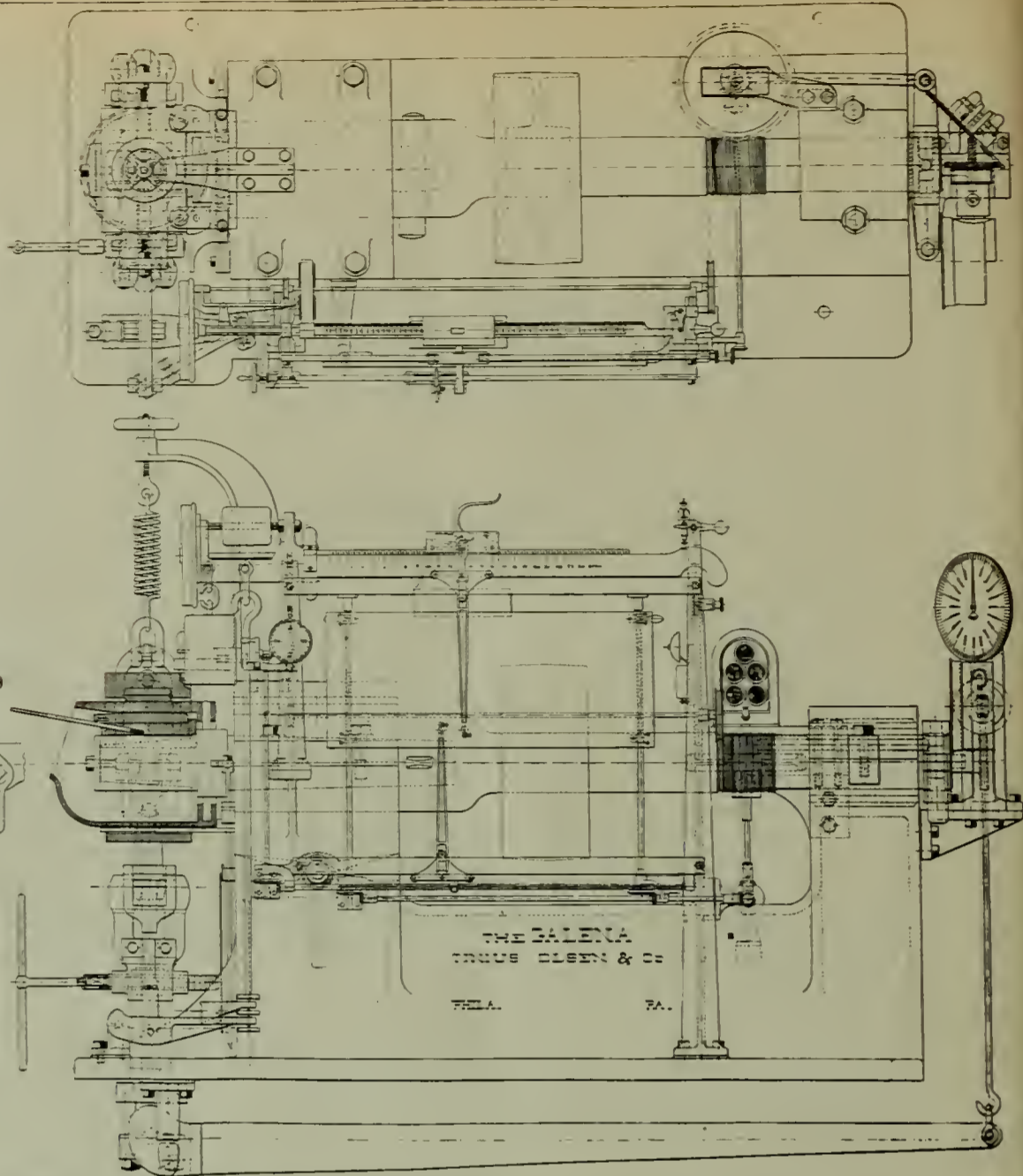
FIG. 10.—GALENA LABORATORY—OIL TESTING MACHINE.
