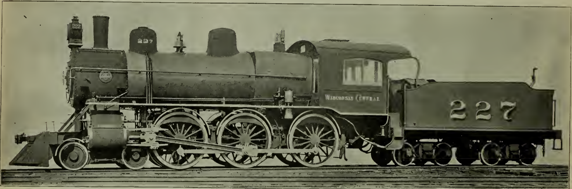
TEN WHEEL PASSENGER LOCOMOTIVE--WISCONSIN CENTRAL RY.
