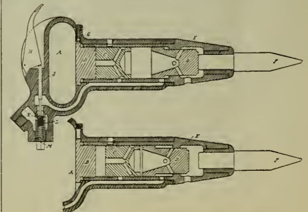
FIG. 2.—DETAILS OF COUNTERBALANCED HAMMER.
