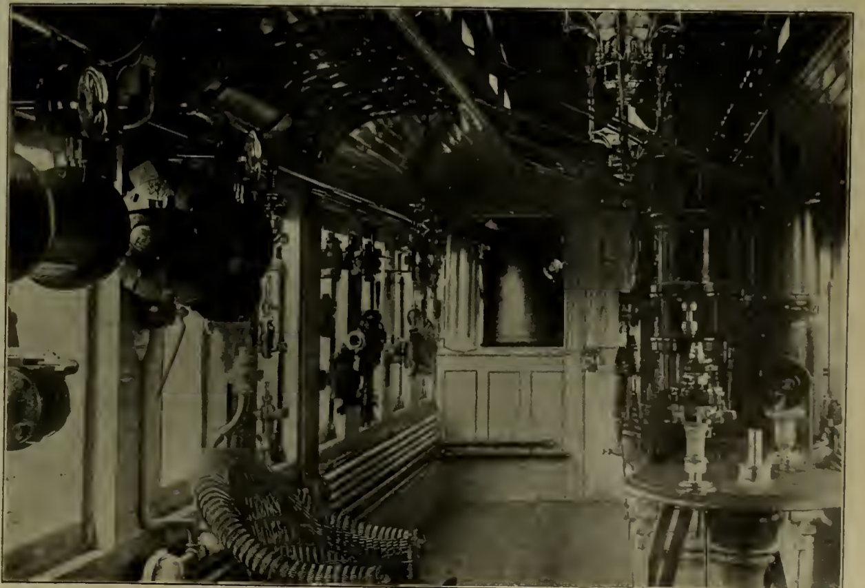
AIR BRAKE INSTRUCTION CAR—N. Y., N. H. & H. RY.—INSTRUCTION ROOM; LOOKING TOWARDS BOILER.
