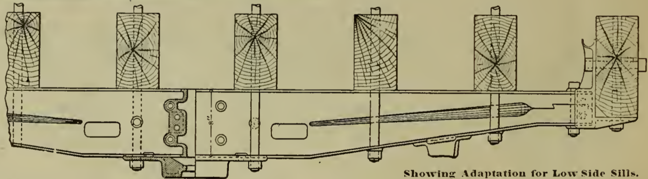
Showing Adaptation for Low Side Sills.
