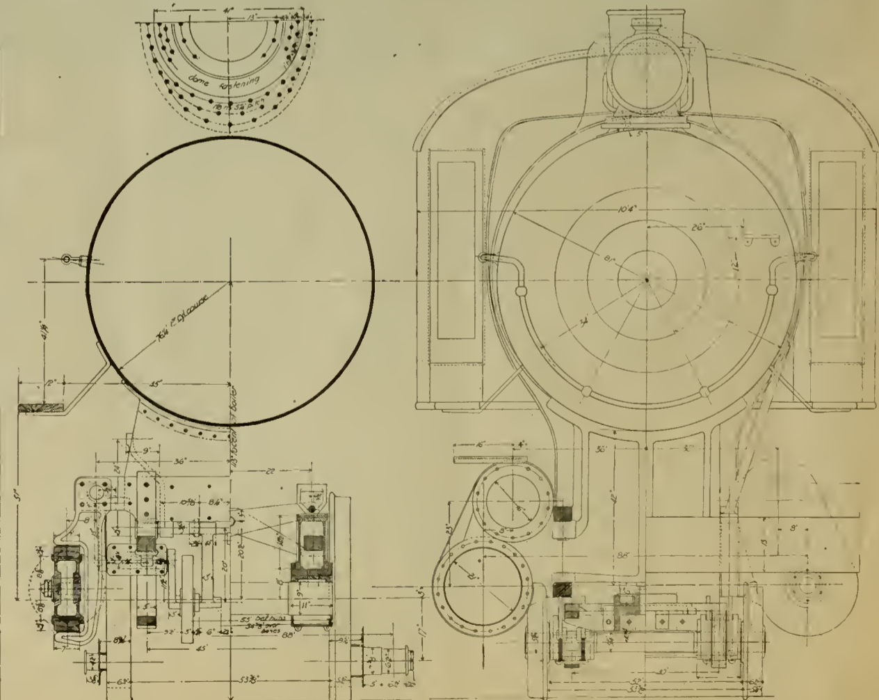
FIG. 7.—HEAVY MASTODON LOCOMOTIVE—GREAT NORTHERN RAILWAY.
