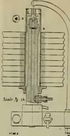
Fig. 5. Loaded Ram for Testing Pressure Gauges.
