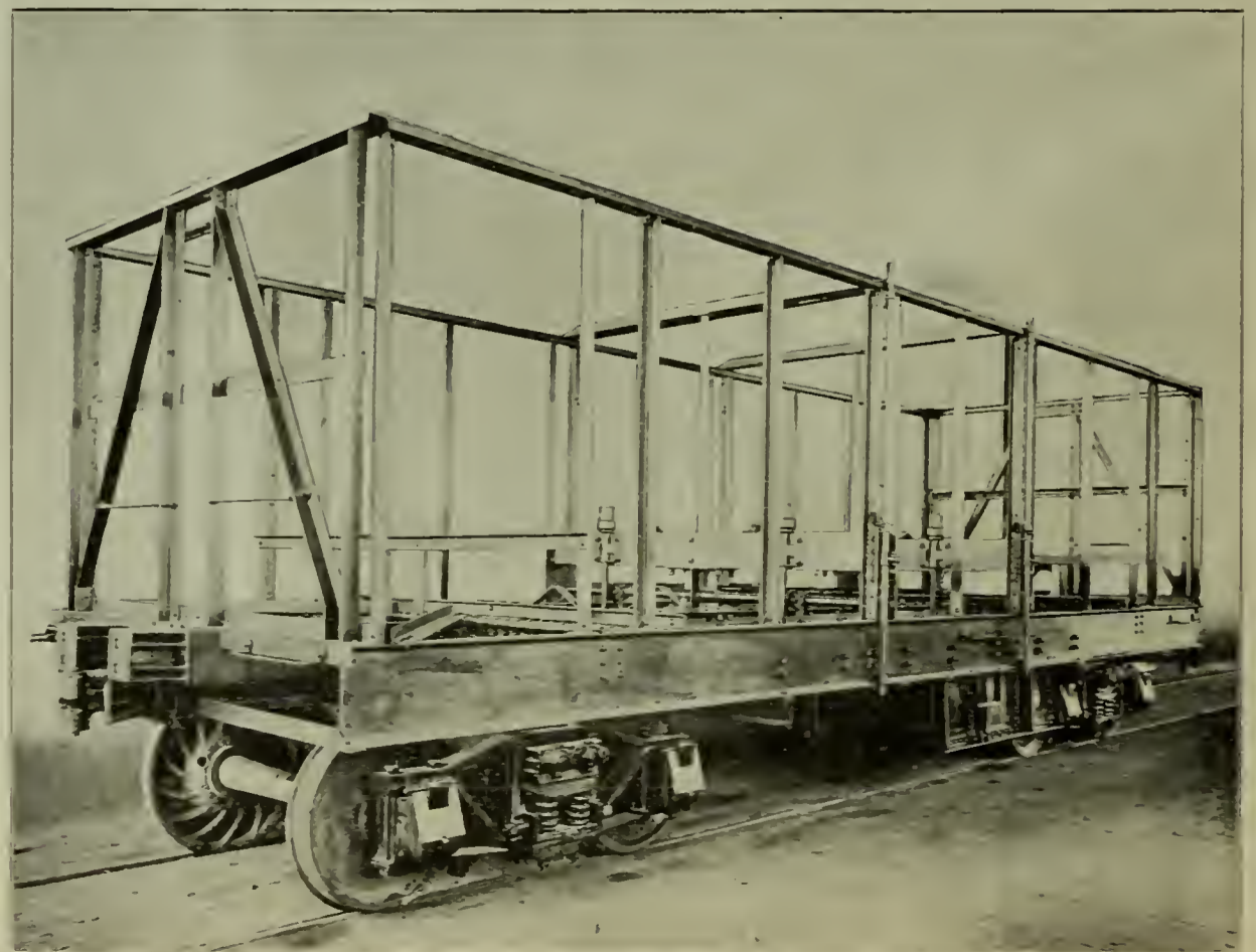
100,000 POUNDS STEEL COAL CAR—NORTHERN PACIFIC RAILWAY—STEEL FRAME.
