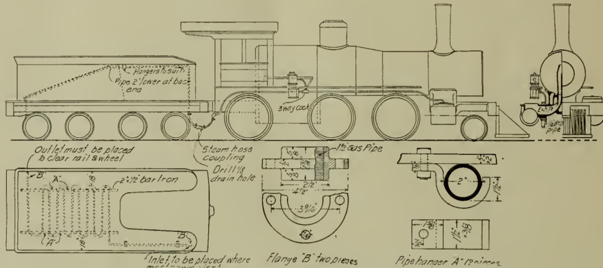
FEED WATER HEATER—NORTHERN PACIFIC RY.
