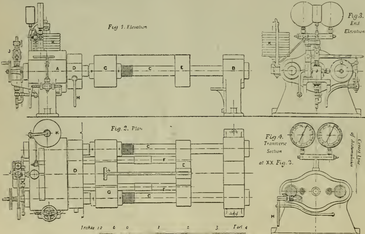
FIGS. 1 TO 4.—TESTING LOCOMOTIVE MATERIALS—MIDLAND RY. OF ENGLAND.
