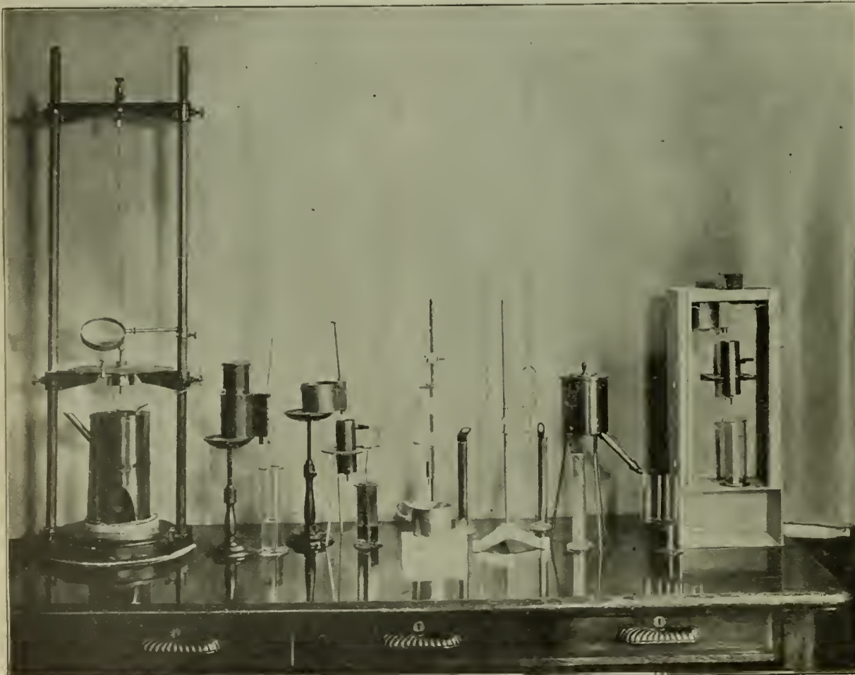
FIG. 12.—GALENA LABORATORY—VISCOSIMETERS.
