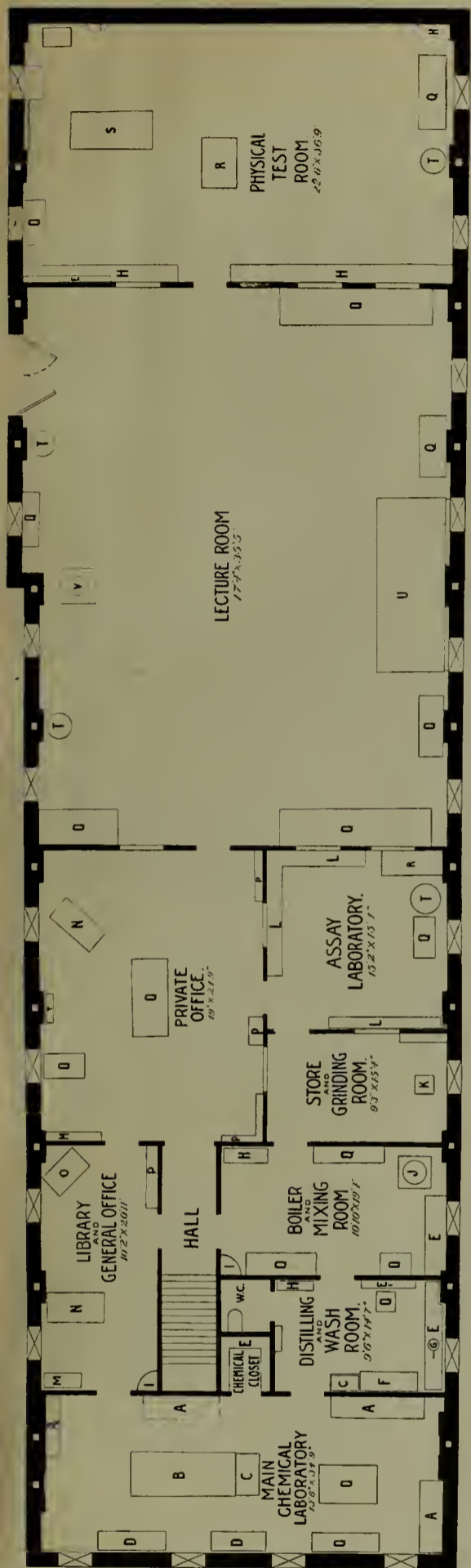
TESTING LABORATORY OF THE GALENA OIL CO., AT FRANKLIN, PA.—FLOOR PLAN.
