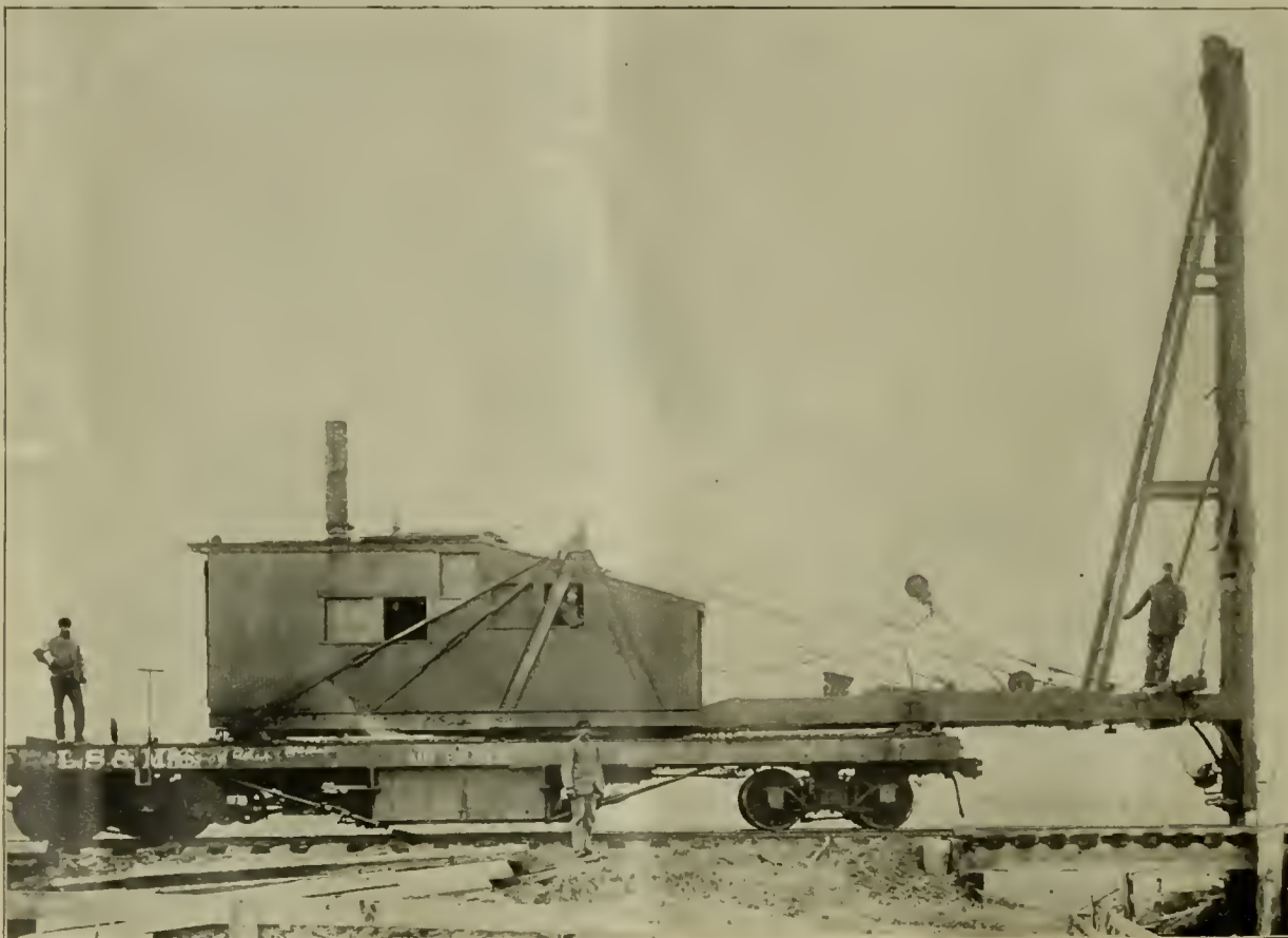
FIG. 4.—PILE DRIVER—L. S. & M. S. RY.—WORKING WITH 16-FT. OVERHANG.
