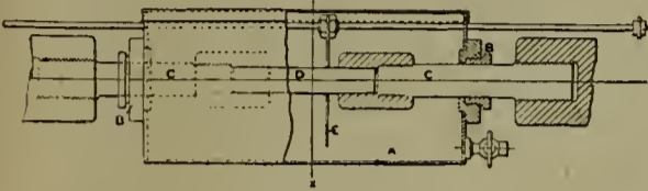
Fig 18 Tensile Test of Locomotive Fire-box Stays under heat
