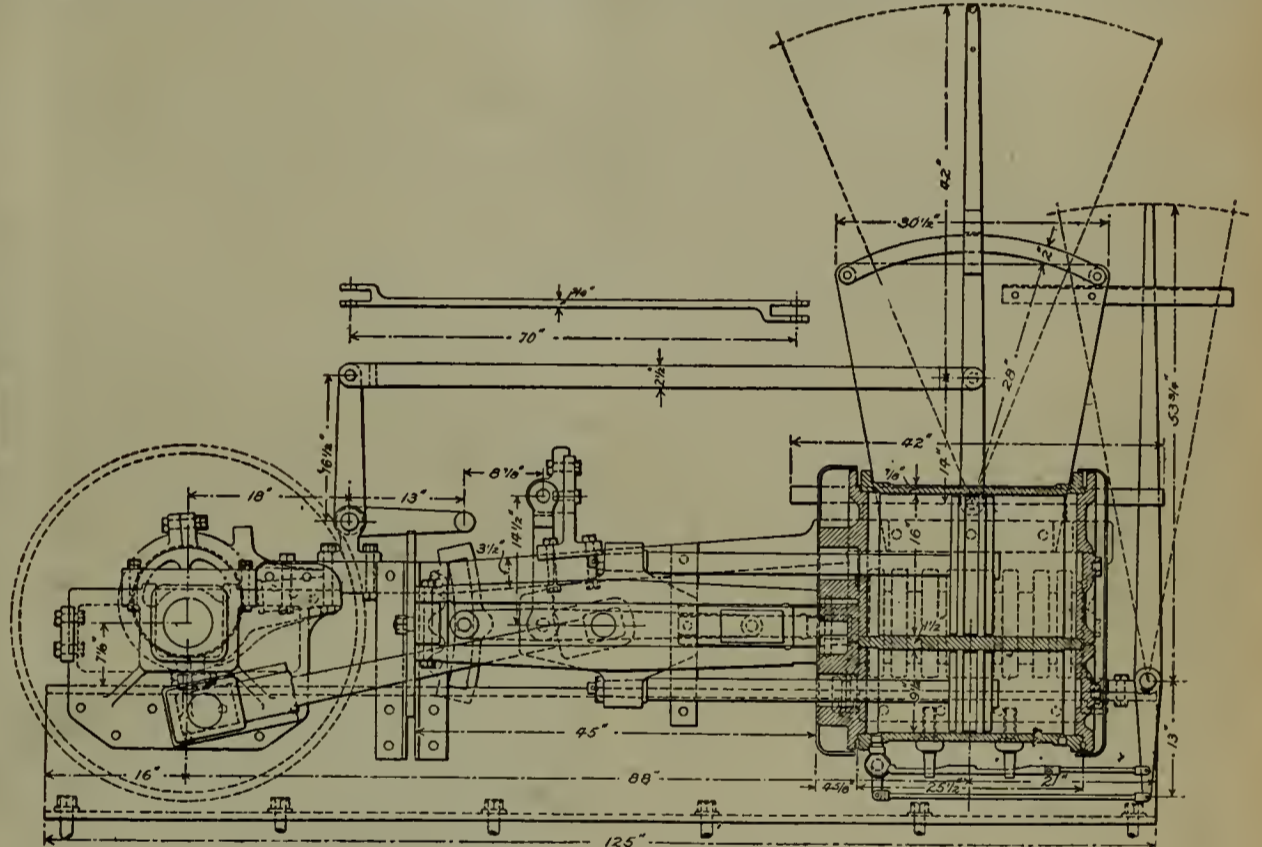
FIG. 6—VAUCLAIN COMPOUND APPARATUS AT PURDUE UNIVERSITY.
