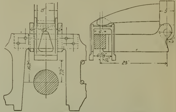
WISCONSIN CENTRAL LOCOMOTIVE DRIVER SPRING ARRANGEMENT.
