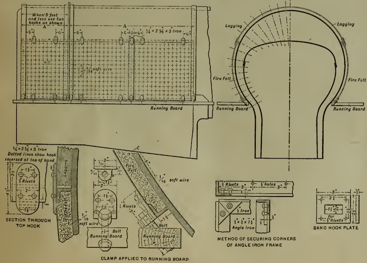
CLAMP APPLIED TO RUNNING BOARD REMOVABLE BOILER COVERING—N. P. RY.
