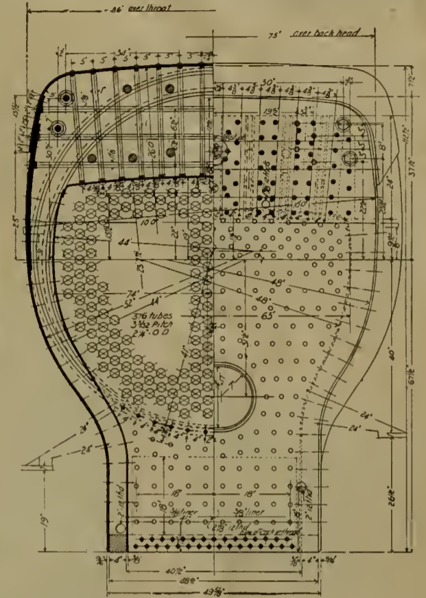
FIG. 5—HEAVY MASTODON LOCOMOTIVE—G.N.RY.
