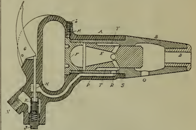
FIG. 1.—DETAILS OF SINGLE HAMMER.
