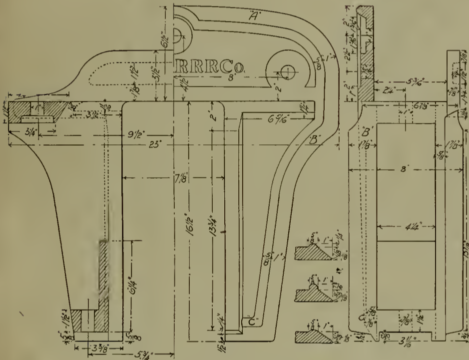
FIG. 2.—PASSENGER CAR PEDESTAL.
