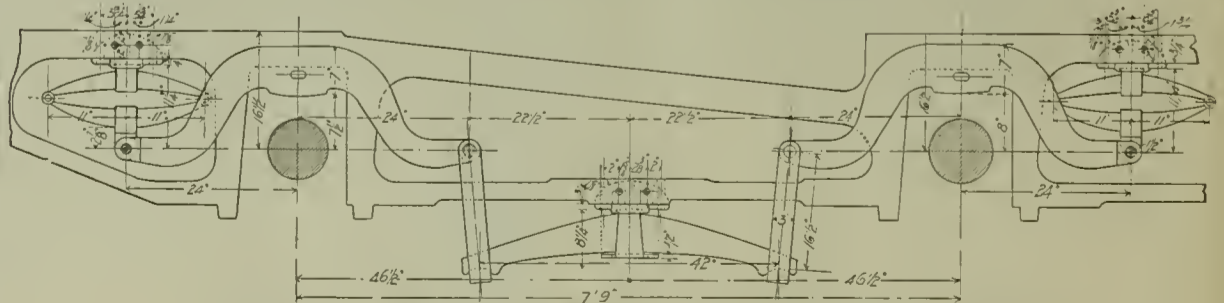
WISCONSIN CENTRAL LOCOMOTIVE--DRIVER SPRING ARRANGEMENT.
