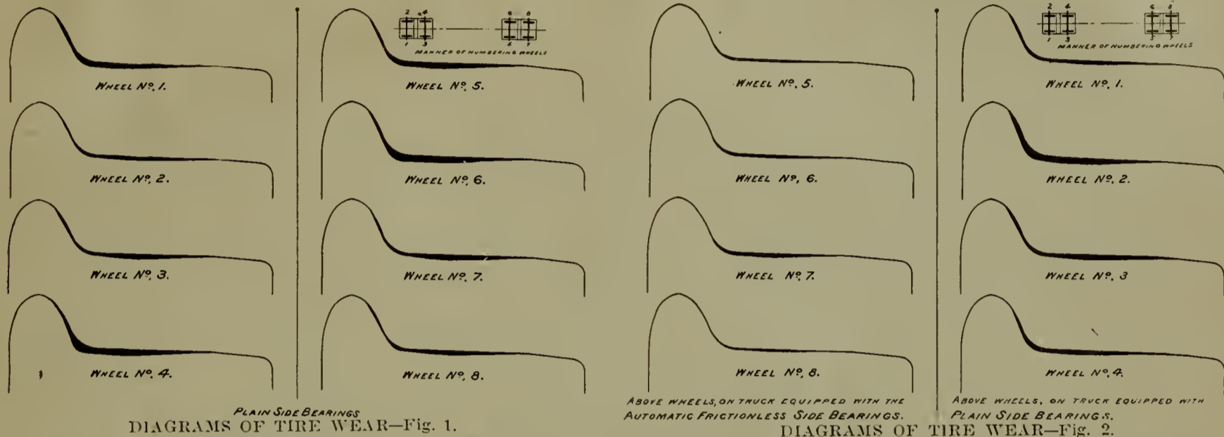
DIAGRAMS OF TIRE WEAR—Fig. 2.
