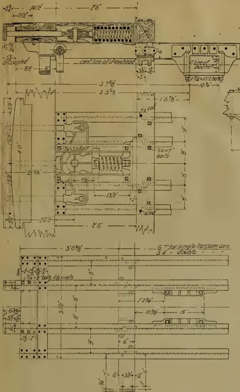
FIG. 3.—GREAT NORTHERN VESTIBULE.—PLATFORM DETAILS.
