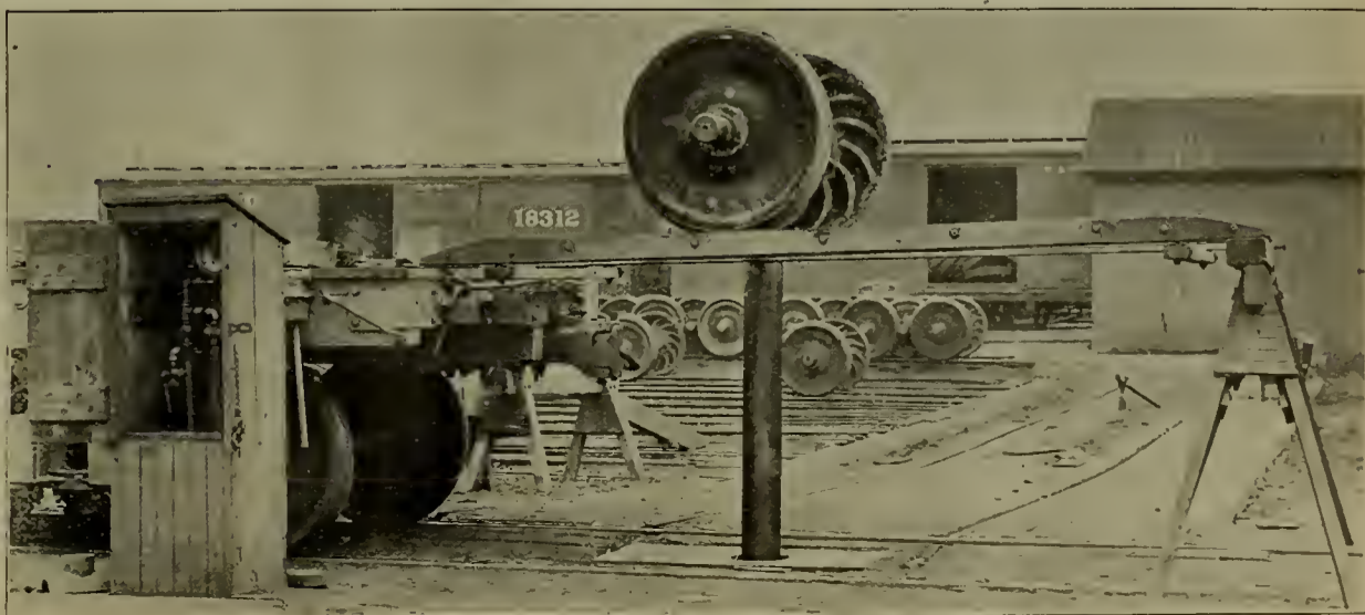
PNEUMATIC WHEEL HOIST—CHICAGO & NORTHWESTERN RAILWAY.
