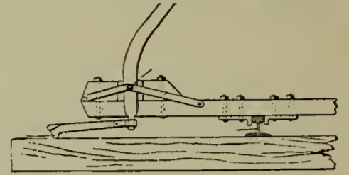
THE SMITH TIE EXTRACTOR AND REPLACER.
