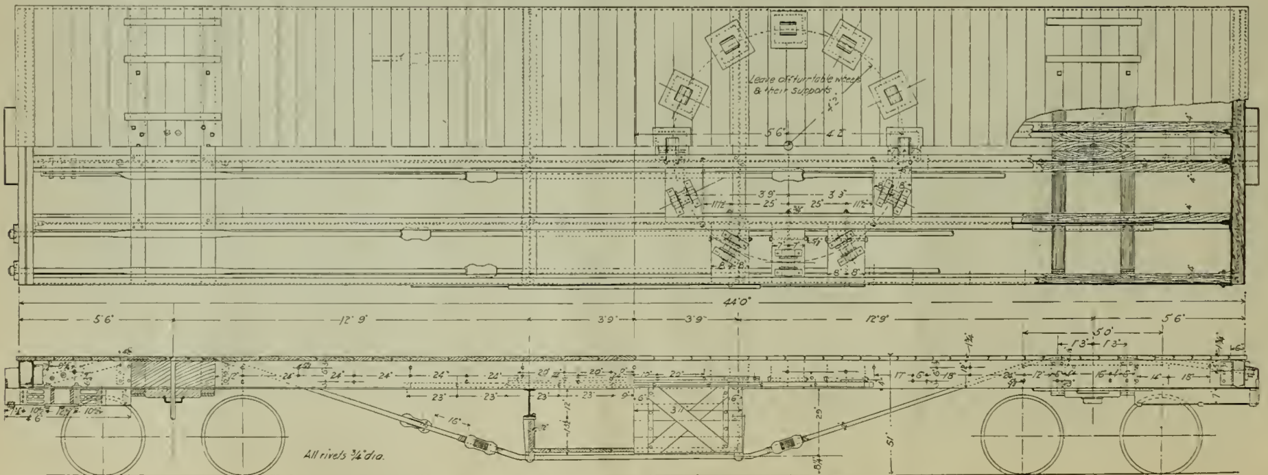
PILE DRIVER CAR—LAKE SHORE & MICHIGAN SOUTHERN RAILWAY.
