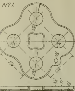
M.C.B. PROPOSED STANDARD SPRING CAPS FOR FREIGHT CAR TRUCKS.
