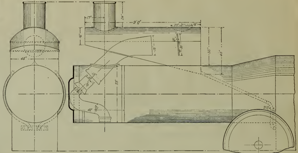
A NOVEL SPARK ARRESTER—NORTHERN PACIFIC RAILWAY.
