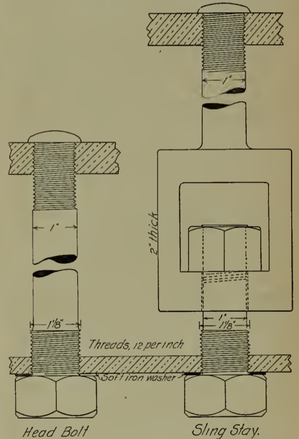
RADIAL AND SLING STAY BOLTS—C. & O. RY.
