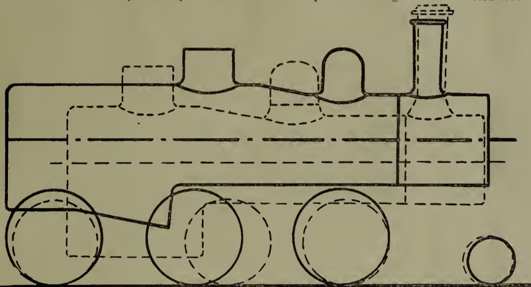
Scale = 3/16" = 1' 19x28 Mogul. 18x24 Mogul.
