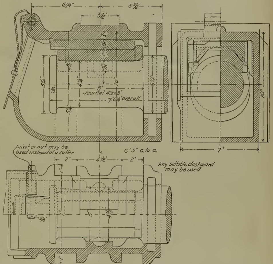
FIG. 3.—JOURNAL BOX AND MAIN PARTS FOR 4 1/4 X 8 IN. JOURNAL.
