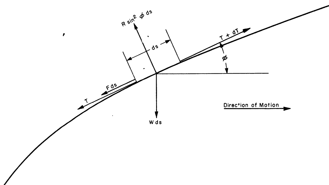
Figure 1 - Forces on an Element of Towing Cable
