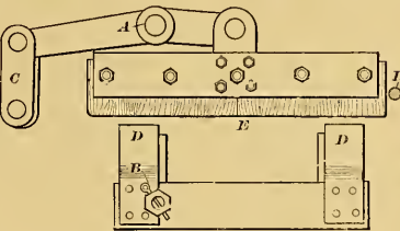
Fig. 4 NORTH HUDSON COUNTY CABLE RAILWAY.
