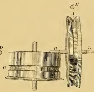
Fig. 4 NORTH HUDSON COUNTY CABLE RAILWAY.
