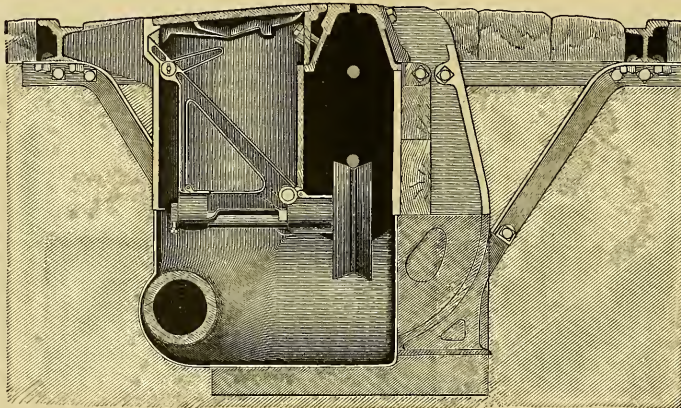
FIG. 5.—CARRYING SHEAVE.
