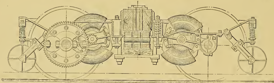
FIG. 4.—ELECTRIC RAILWAY TRUCK—ELEVATION.
