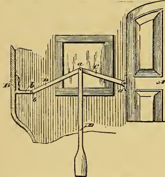
Door closed, fastener in position, weight suspended from the toggle joint, holding it closed.
